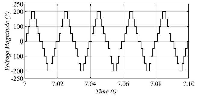
FIGURE 10. Output waveform of 9-level MLI operating on novel PWM technique.
