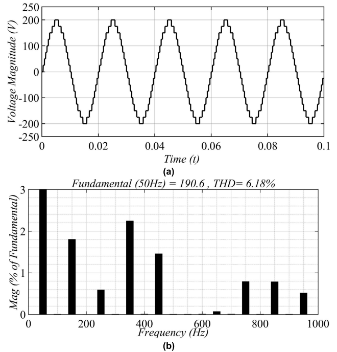
FIGURE 12. (a) Output waveform of 17 level SLMHB-MLI (b) THD of the proposed topology; operating on novel PWM technique.
