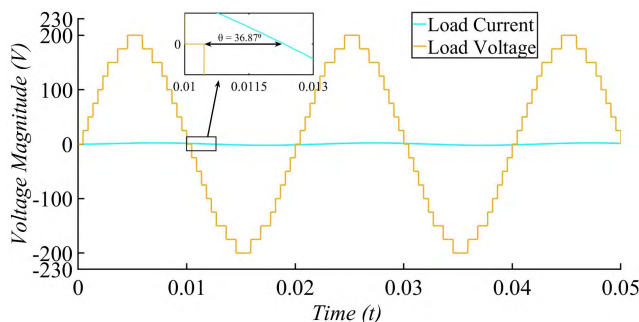
FIGURE 21. Simulated result of the load voltage and load current at 0.8 PF.
